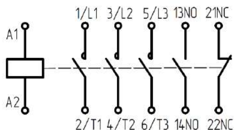
LC1E40...LC1E95
