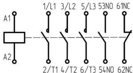
LC1E120...LC1E630
