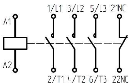
LC1E0901...LC1E3201
