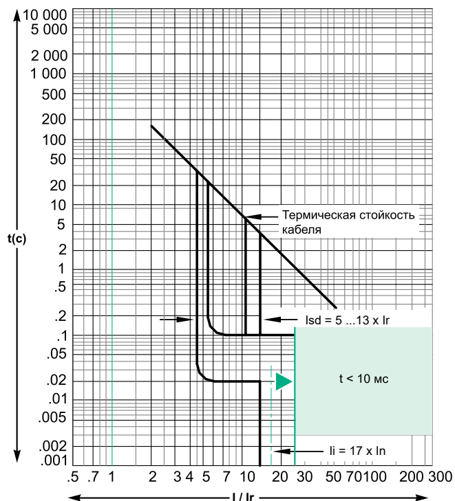
GM6L 320 A
