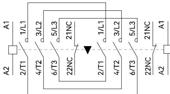
MC2Kxx01xx
