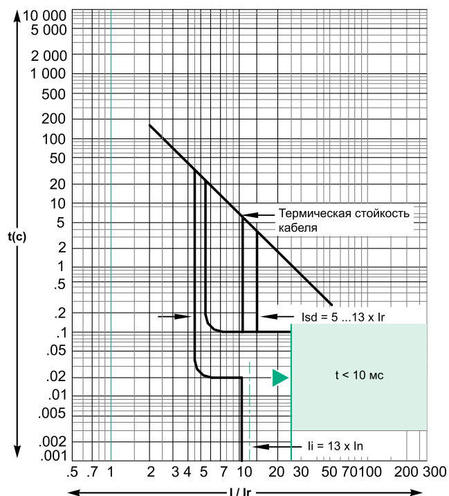
GM6L 500 A
