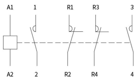
MC2Kxx01xx
