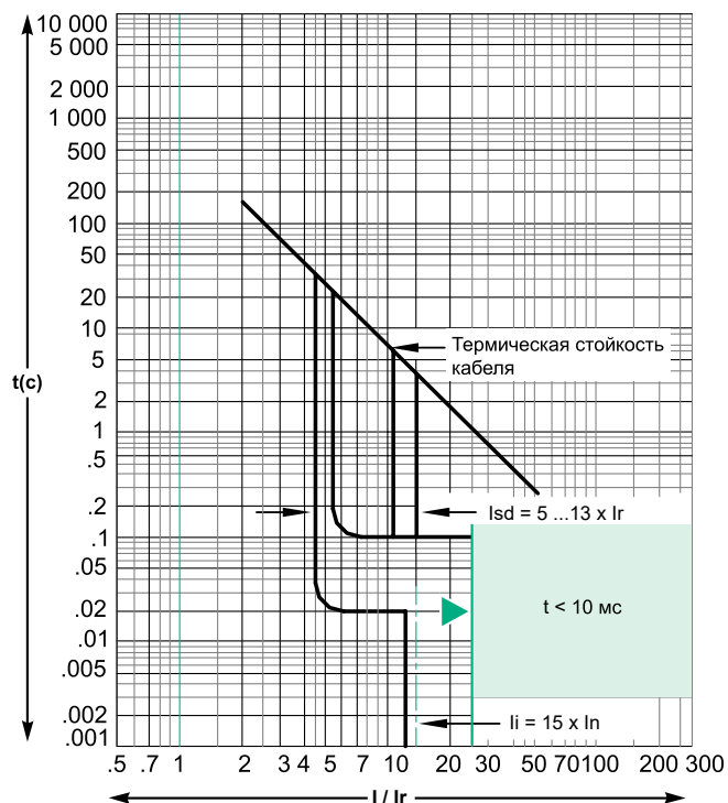
GM6L 500 A
