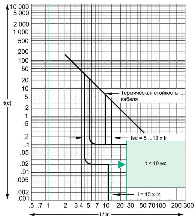
GM6L 320 A
