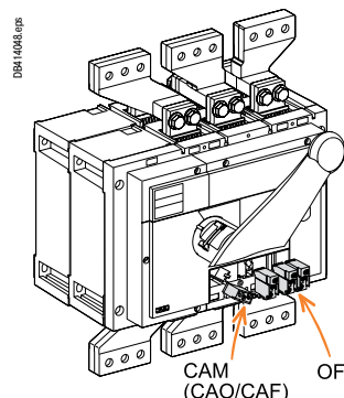
Compact INS/INV2000 - 2500
